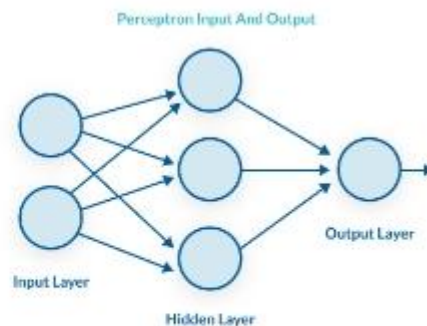
Figure 3. Simplified SLP with 1 hidden layer
