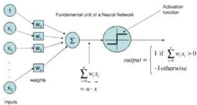
Figure 2. A Single Layer Perceptron
