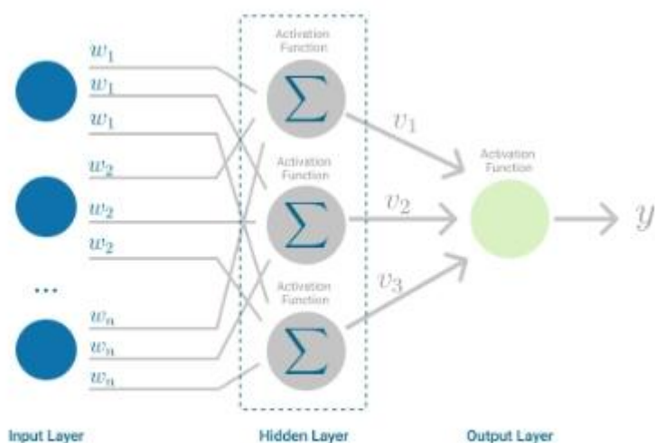
Figure 5. Multi-Layer Perceptron
